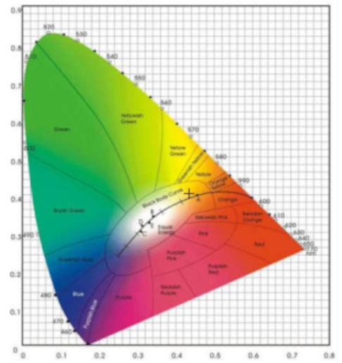
CIE1931
